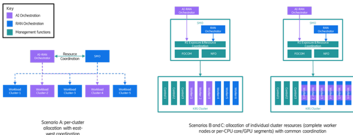
Figure 1. AI RAN Sharing Scenarios
