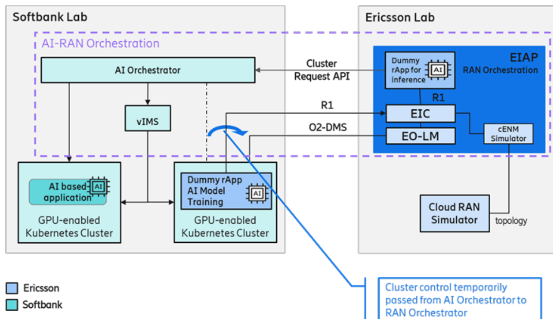
Figure 2. AI-RAN Lab Demonstration Setup
